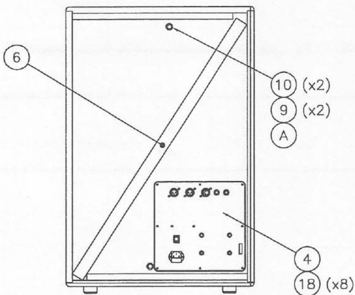
BACK VIEW W/O DOLLY BACK & CASTERS
